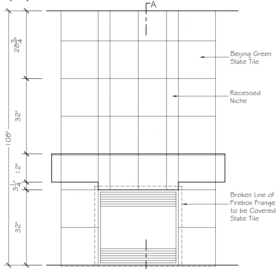
2 Fireplace Front Elevation Scale: 1/2" = 1'-0"
