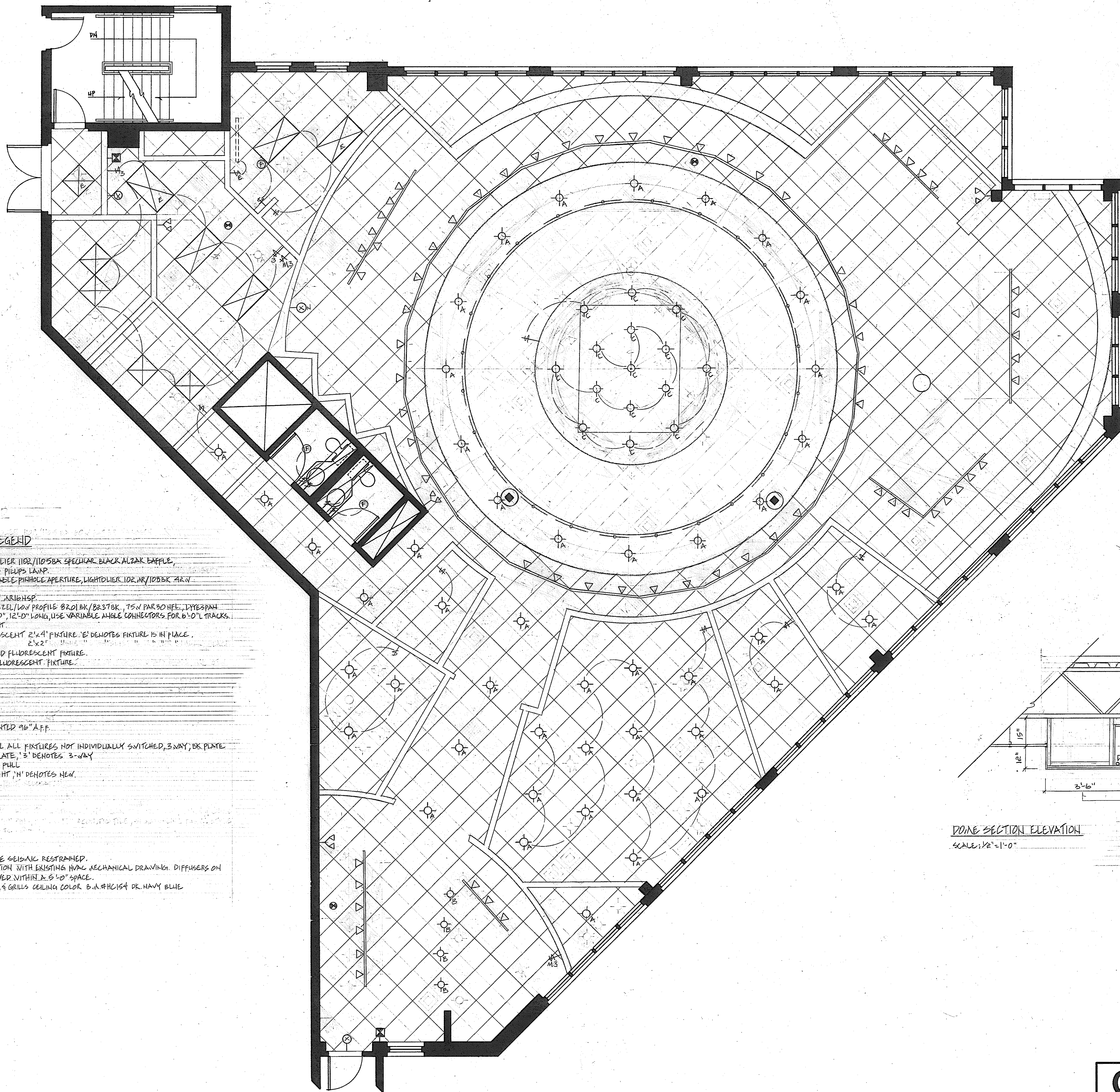
REFLECTED CEILING PLAN SCALE: 1/4" = 1'-0"
